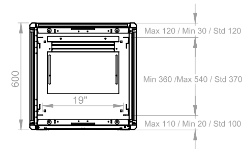
Max/std/min equipment mounting distance
