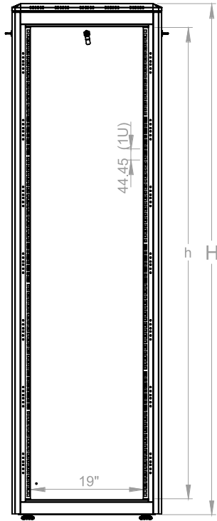
Dimensions in width and height
