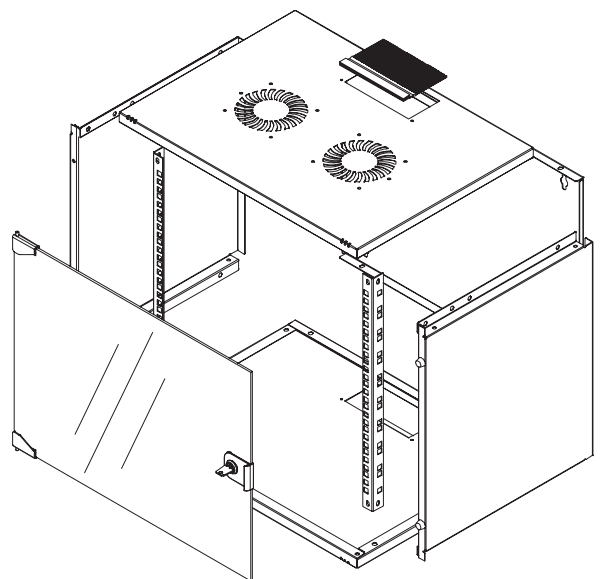
Exploded view
